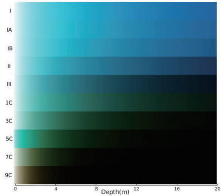
Fig. 3 Simulation results for light absorption underwater.
