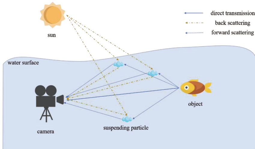
Fig. 2 General view of the underwater image formation process.
