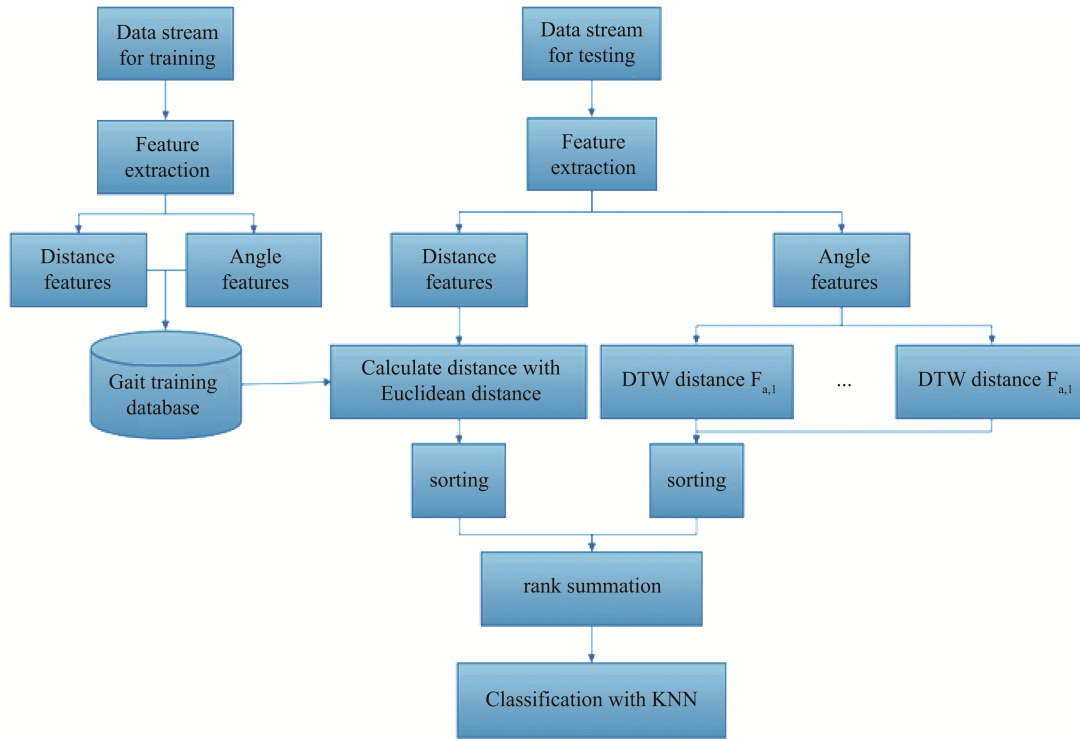
Fig.5 System Architecture with Score-level Fusion
